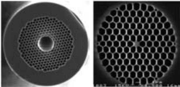
(Left) Scanning electron micrograph of an ultra-low-loss hollow-core photonic crystal fiber (PCF) with a core diameter of 20 \mu\text{m} . (Right) highly nonlinear PCF with a solid core, 1.1 \mu\text{m} in diameter.
