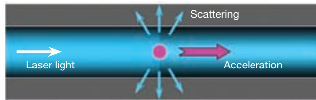
The particle will strongly scatter the light and experience constant acceleration (in the absence of fiber loss).
